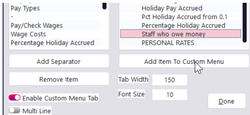
Figure 3: Custom Reports
